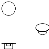
Ø 600 x 420H - Ø 1000 TOP W/ ACCESS HATCH
