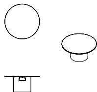
Ø 800 x 730H - Ø 1600 TOP W/ ACCESS HATCH
